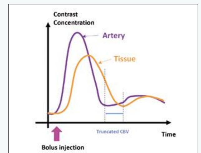
Figure 2: Tissue vs. artery concentration-time curves
