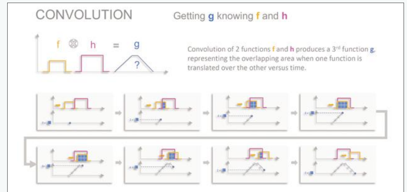
Figure 4: Understanding how convolution product works
