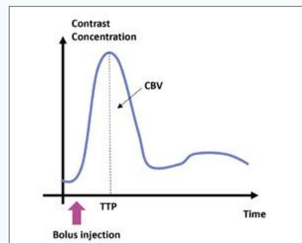
Figure 1: Typical concentration-time curve
