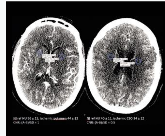
Figure 7: CNR of CTP images, calculated as the difference between the ROI values within normal tissue and within the ischemic area divided by the standard deviation (SD) of the ischemic ROI value
