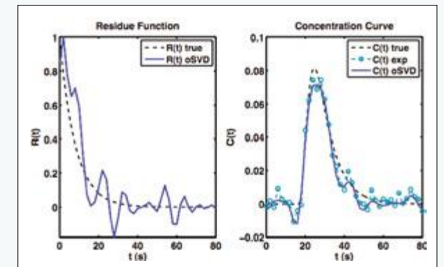
Figure 10: Residue function and concentration curve from oSVD (blue lines) compared to true curves (dotted line) using digital phantom data. Adapted from [23]
